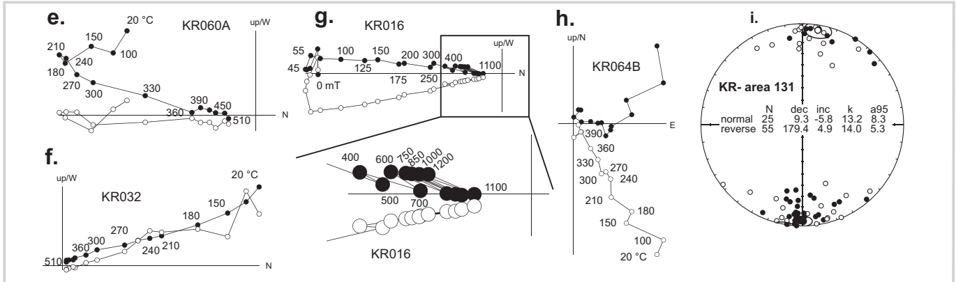
Figure 3. Paleomagnetic results. a–c and e–h Representative demagnetization behaviors observed in the section of Areas 105 (KS section) and 131 (KR section) respectively. Solid (open) points are projections on the horizontal (vertical) plane. d and i. Stereographic projections of ChRM directions. Solid (open) points are projections on the lower (upper) hemisphere. Mean of normal and reversed directions are indicated by larger points and given in central table (dec, declination; inc, inclination; k, precision parameter; a_{95} , 95% confidence cone). c. Typical thermal demagnetization path (steps given in °C) going to reversed direction treated by great circle analysis (McFadden and McElhinny, 1988). g. Typical AF demagnetization with biasing above 200 Oersted (see enlarged inset) interpreted to result from gyroremanence acquisition during AF treatment. h. Widely outlying direction interpreted as transitional.
