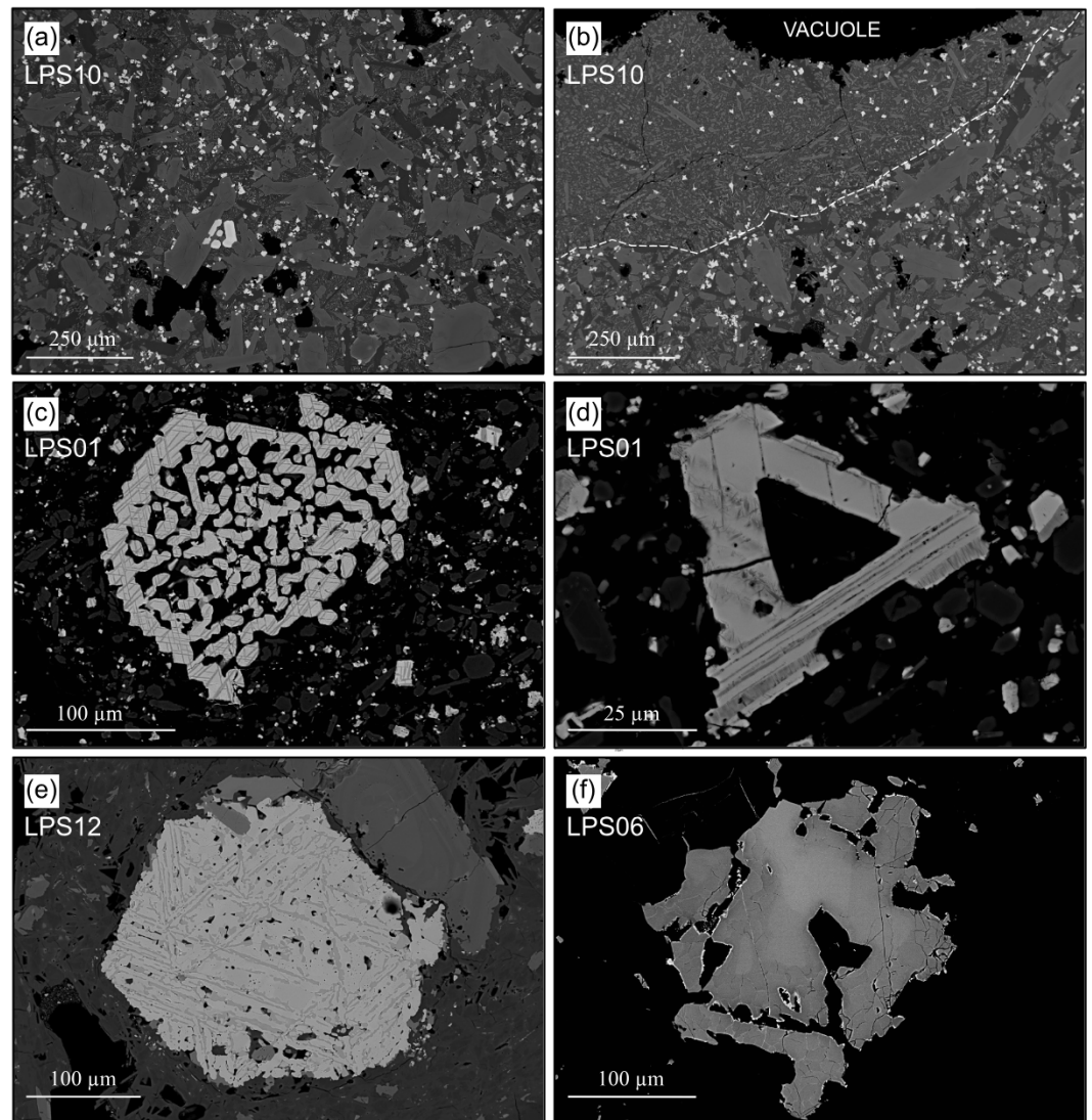
Figure 2. Field-emission scanning electron microscope detail images of different representative samples. (a) General view of the distribution of opaque minerals in sample LPS10: the larger crystals in the central area display darker chromite (Chr) cores surrounded by brighter titanomagnetite rims. (b) Detail of sample LPS10 with two crystallization stages of the magma: in the upper part, a zone depleted in opaque minerals is observed, with smaller crystals. (c) Skeletal titanomagnetite crystal with Trellis-type exsolved ilmenite lamellae in sample LPS12, an example of high-temperature oxidation stage C3 (Haggerty, 1976). (d) Skeletal opaque crystal from sample LPS01: the ilmenite lamellae have transformed into alternating sigmoidal lenses of rutile and titanohematite, characteristic of C4 oxidation stage. (e) Euhedral crystal pseudomorphed to hematite (host phase) with exsolved lamellae of pseudobrookite in sample LPS12, corresponding to stage C7. (f) Skeletal opaque crystal from sample LPS06: thin, curved cracks related to volume changes, along with progressively darker crystal edges due to iron depletion, indicating intense low temperature oxidation.
