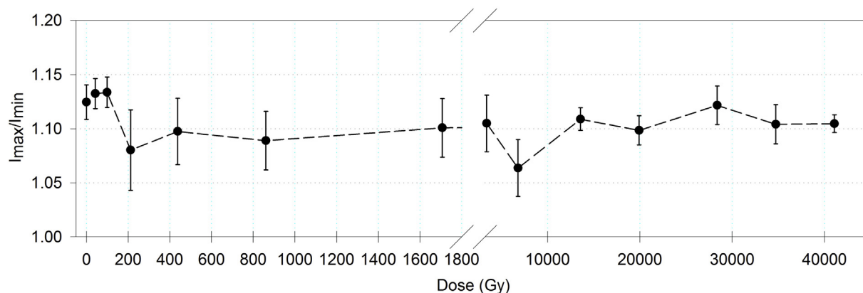
Fig. 6. Evolution of the I_{\max}/I_{\min} ratio measured in ATD6-92 with the irradiation dose. The error on the ratio is derived from the standard deviation ( 1\sigma ) associated to the evaluation of I_{\max} and I_{\min} , which are taken as mean I_{\max} and I_{\min} values from three successive angles.
