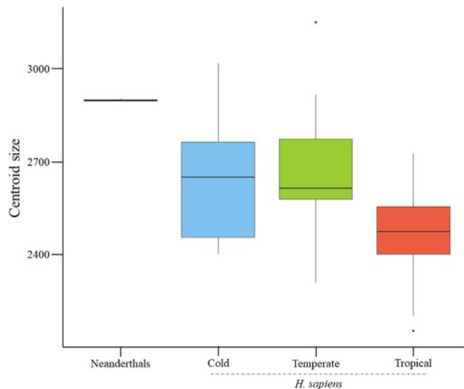
Figure 3. Boxplots comparing the centroid size of the Neanderthals and the Homo sapiens sample grouped by latitude. Neanderthals are significantly larger ( p < 0.05 ) than tropical and temperate H. sapiens , but no differences were found between them and cold-adapted H. sapiens .
