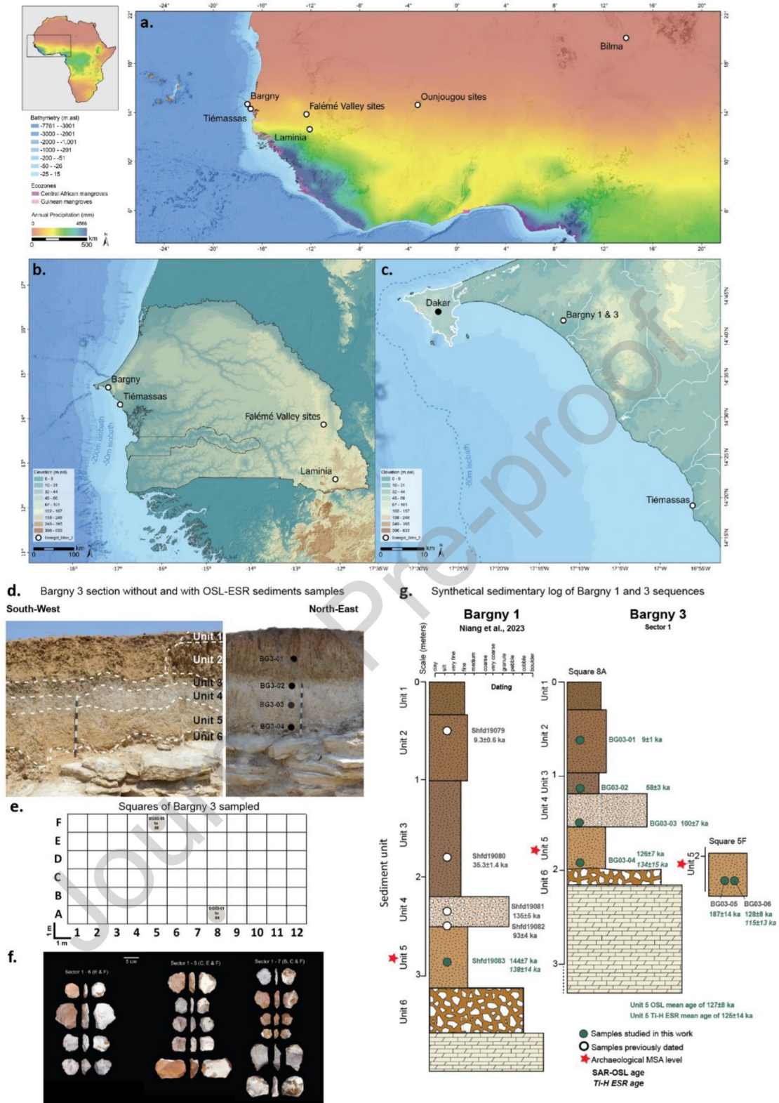
Figure 1: Geographical location of the MSA sites presented and discussed in this work and Bargny 1 and 3 sequences. a: Location of the sites at west African scale and at b: regional scale; c: Location of Bargny sequences; d: view of the main sections of Bargny 3 without and with the samples; e. plan of Bargny 3 presenting the location of the dating samples in this work; f: example of MSA artifacts from Unit 5 of Bargny 3; g: synthetic sedimentary log from Bargny 1 and 3 and associated dating results.
