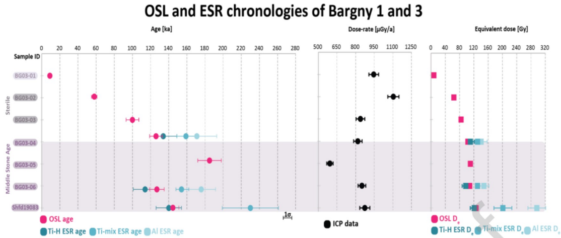
Figure 2: Overview of the OSL-ESR data (ages, dose rate and equivalent dose) collected from Bargny 1 and 3 sequences. Numerical values are given in Table 1 . Errors are 1\sigma .
