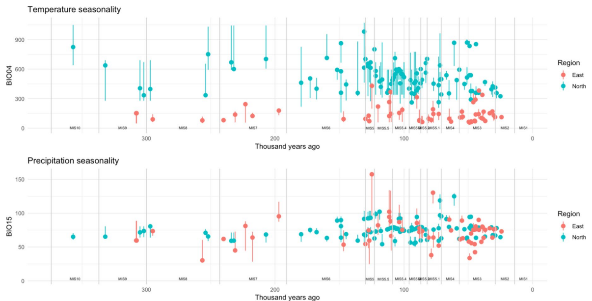
Fig. 3. Temperature (bio04; °C) and precipitation (bio15; mm) seasonality experienced during Middle Stone Age occupations in eastern (red) and northwestern (blue) Africa at the mid-age (circles) and across the date range (lines). Marine Isotope Stages are denoted, based on Lisiecki and Raymo 80 .
