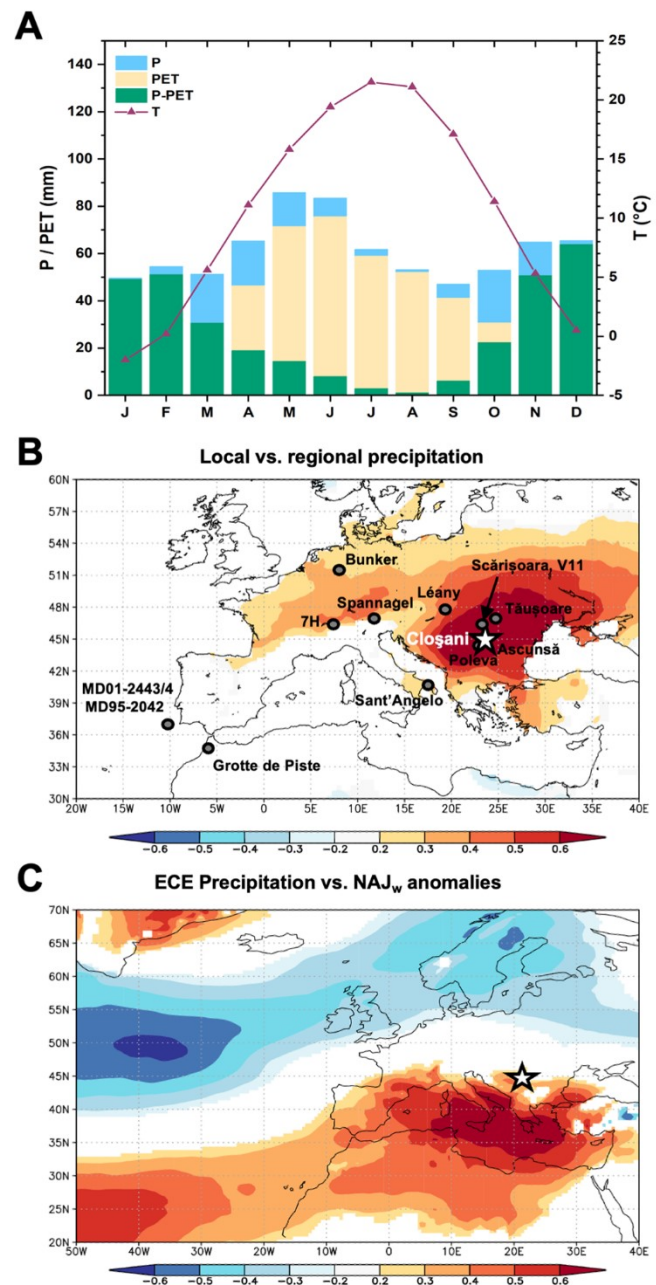
Fig. 1 | Locations and present-day regional climatology. A Monthly climate data in SW Romania from meteorological stations Târgu Jiu (T) and Drobeta/Turnu Severin (DTS) averaged for the period 1961–1990 CE. B Location of Cloșani Cave (white star) as well as other sites discussed in this study (grey symbols). Background shows the spatial correlation of averaged Oct–Mar precipitation from five GHCNm stations near Cloșani Cave with averaged Oct–Mar CRU TS4.07 precipitation data for the years 1901–2018 CE. C Same as background in B but compared to NAJ w strength represented by 850 hPa zonal wind anomalies (relative to 1991–2020 CE) obtained from the ERA5 reanalysis dataset. Spatial correlation maps were created with KNMI Climate Explorer 48 . Maps in B , C show only significant correlation patterns ( p < 0.1 ).
