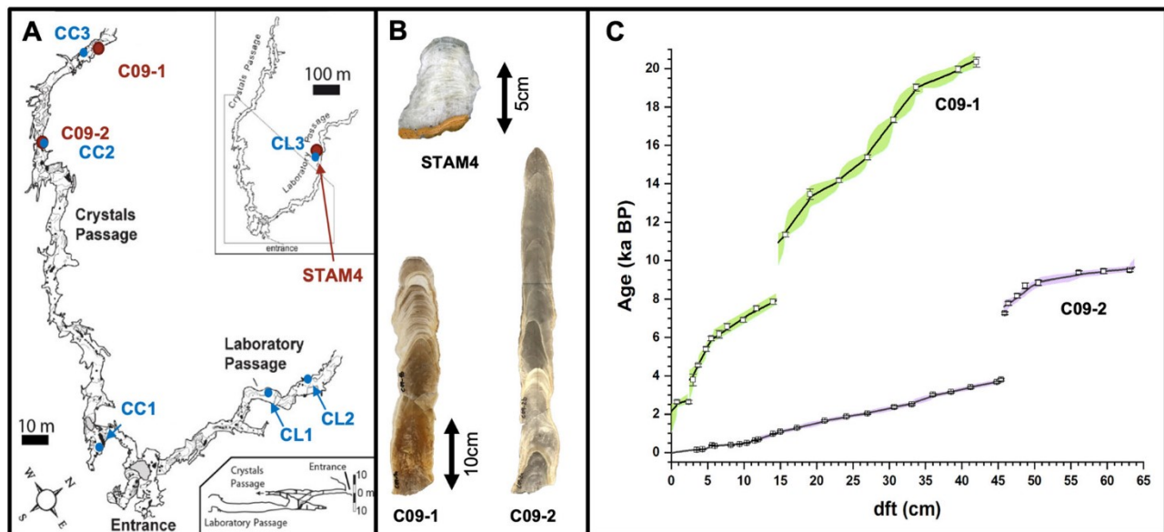
Fig. 2 | Cave setting and speleothem samples. A Map of Cloșani Cave with locations of stalagmites C09-1, C09-2 and STAM4, as well as the locations of the drip sites CC1-3 in the Crystals Passage and CL1-3 in the Laboratory Passage. B Scans of
