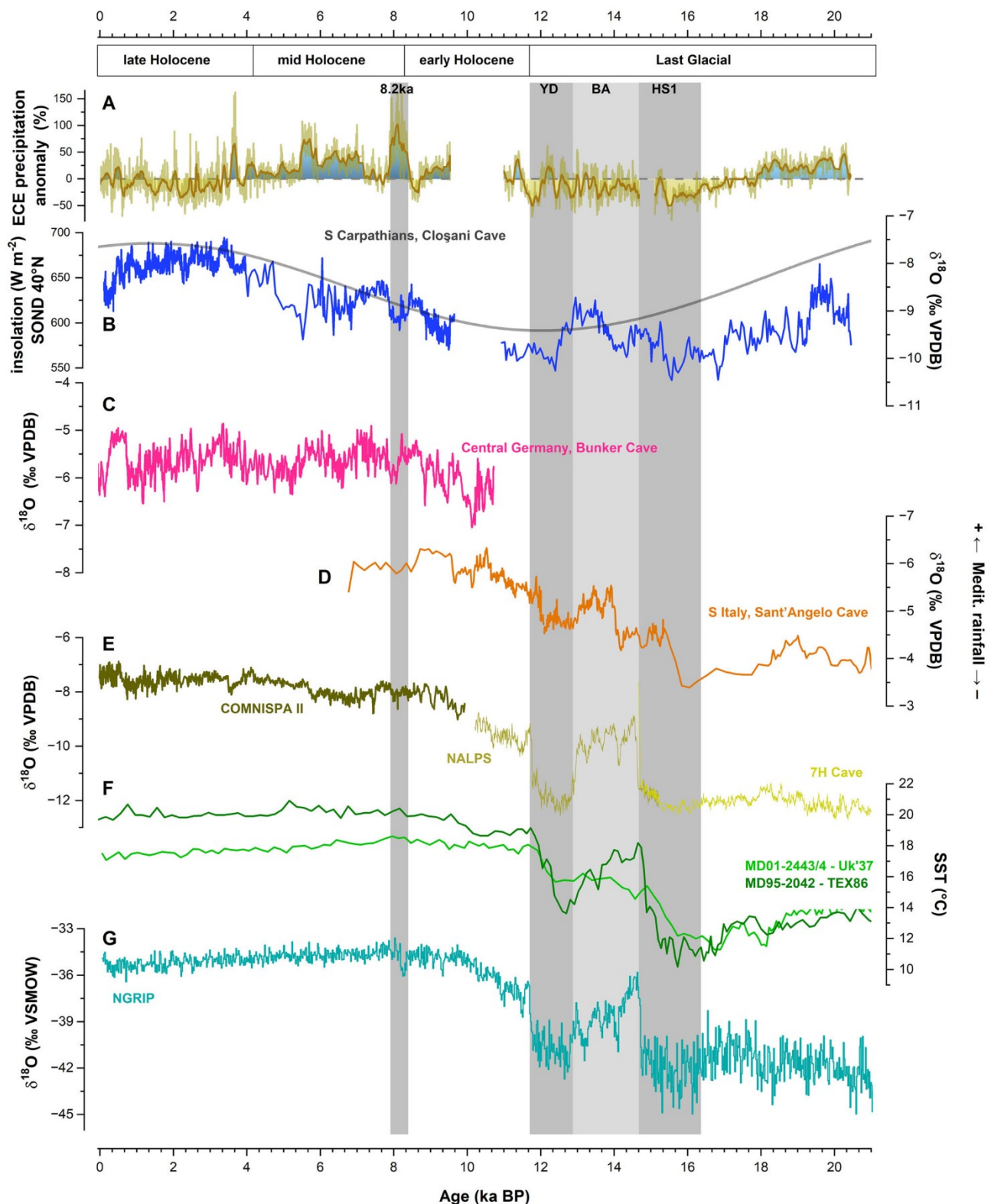
Fig. 5 | Eastern Central Europe hydroclimate and atmospheric circulation during the past 20 ka. The figure shows A Composite Cloșani Cave f_{Ca} derived precipitation anomalies relative to the period 1873–2010 CE. The dark yellow line shows a 100 yr running mean. B Cloșani Cave composite \delta^{18}O record (blue), and September to December insolation at 40^{\circ}N . Both records are compared to European climate records from top to bottom: C Bunker Cave composite \delta^{18}O record W Germany 47 ,
