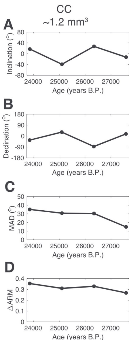
Figure 12. Summary of magnetic directions, maximum angular deviation (MAD) and \Delta\text{ARM} values as a function of age for the Crevice Cave (CC) samples. Shown are plots for (a) inclination, (b) declination, (c) MAD and (d) \Delta\text{ARM} .
