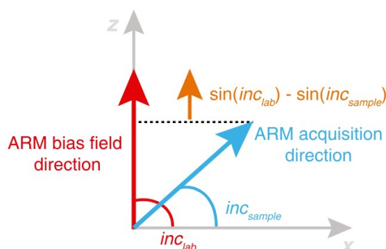
Figure 2. Diagram showing how the \Delta\text{ARM} is calculated. The red arrow indicates the applied field direction, \text{inc}_{\text{lab}} , and the blue arrow indicates the angle associated with the direction of the anhysteretic remanent magnetization (ARM) acquisition by the sample, \text{inc}_{\text{sample}} . The \Delta\text{ARM} parameter quantifies the average difference between these two directions across multiple ARM applications.
