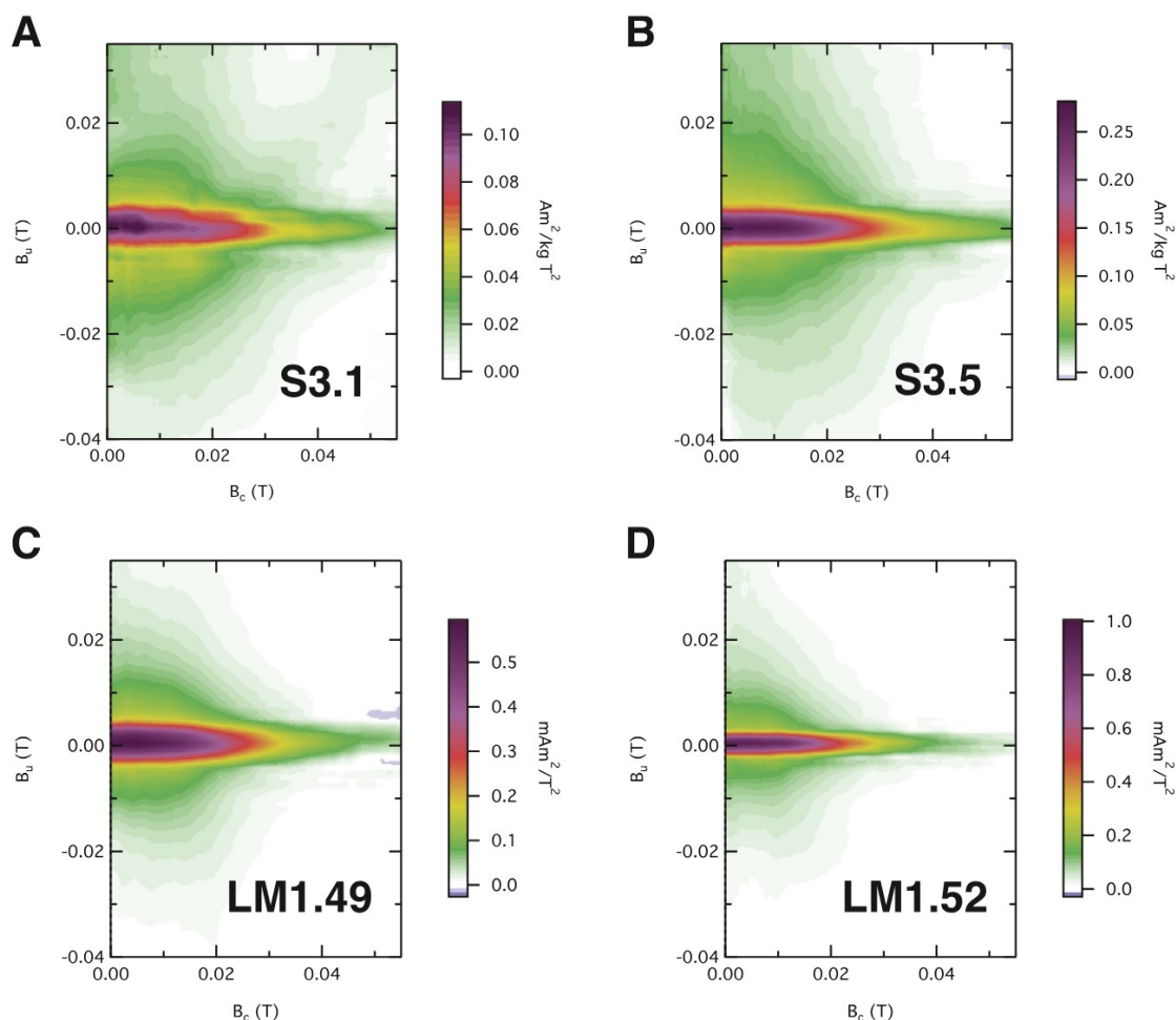
Figure 3. First-order reversal curve (FORC) diagrams for select PD and LM samples. FORC diagrams for samples (a) S3.1, (b) S3.5, (c) LM1.49, and (d) LM1.52. All four samples exhibit similar features on the FORC diagrams, indicating the presence of single-domain and vortex state magnetic carriers. The difference in signal strength between samples from the same speleothem coupled with the overall similarity of features in the FORCs indicate that the concentration of magnetic carriers varies across the samples.
