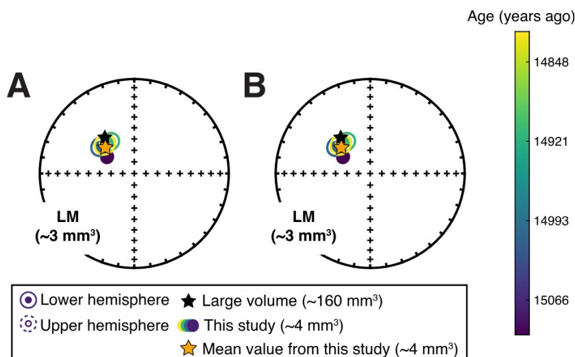
Figure 13. Comparison between high coercivity directions measured with traditional paleomagnetic techniques and by superconducting quantum interference device (SQUID) microscope for Lapa dos Morcegos (LM) samples. (a) Equal area stereographic projections showing all directions obtained from LM1. (b) Equal area stereographic projections showing directions with samples that presented \Delta ARM < 0.047 from the same samples as (a). No samples were excluded by this selection criterion in this case. Black star is the measurement for this sample using traditional paleomagnetic techniques ( \sim 1,600 \text{ mm}^3 ), circles are the SQUID microscope results from this study with color scales indicating the ages of the samples, and yellow star is the average direction of the results from this study ( \sim 4 \text{ mm}^3 ).
