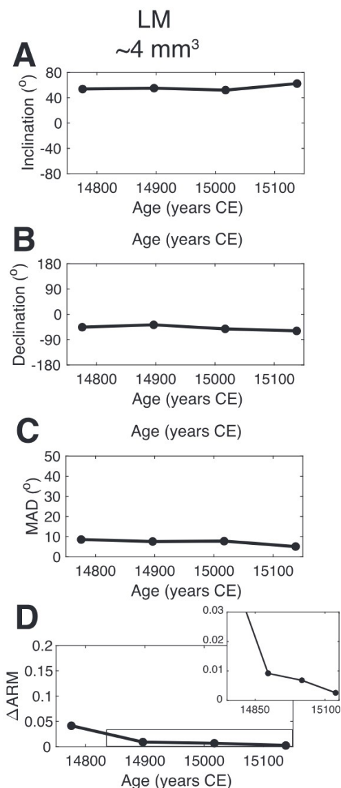
Figure 10. Summary of magnetic directions, maximum angular deviation (MAD) and \Delta ARM values as a function of age for the Lapa dos Morcegos (LM) samples. Shown are plots for (a) inclination, (b) declination, (c) MAD and (d) \Delta ARM , including an inset of the \Delta ARM values.
