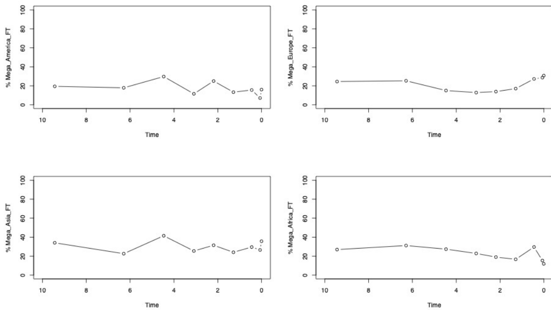
Fig. S23. Megafauna functional types evolution over the last 10 Ma. Percentage of the total functional types belonging to megafauna by continent is plotted against time for the last 10Ma.
