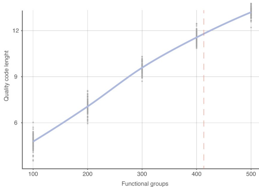
Fig. S19. K-means sensitivity analysis. Quality code length (measure of modularity) is plotted against the number of modules obtained from the network analysis for all k-means randomization (see methods). Dashed red line represents the number of modules used for the analysis (405).
