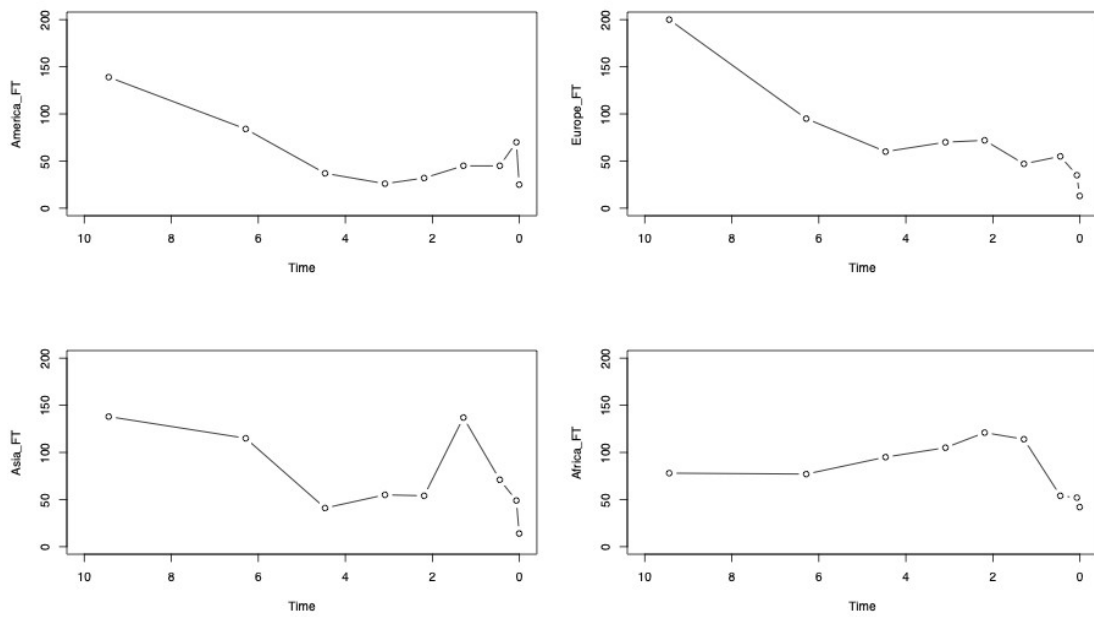
Fig. S22. Functional types evolution over the last 10 Ma. The total number of functional types by continent is plotted against time for the last 10Ma.
