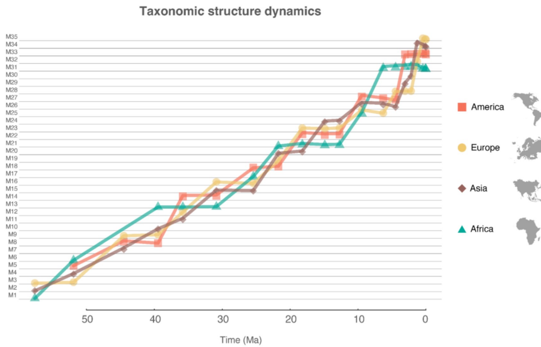
Fig. S1. Large herbivore' taxonomic structure dynamics. Taxonomic structure trends in the different continents are plotted by colors against time in Myrs. Shapes indicate time bins in each continent. Modules (M) derived from network analysis show the functional structure succession in each continent.
