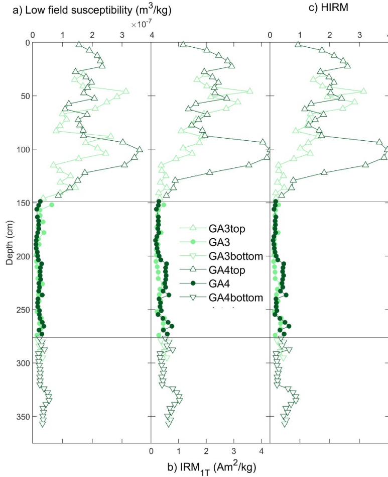
Figure 9. Magnetic parameters of GA3 and GA4 with depth. (a) Low magnetic field susceptibility; (b) IRM_{1T} and (c) HIRM, defined as (IRM_{1T} + IRM_{0.33T})/2 .
