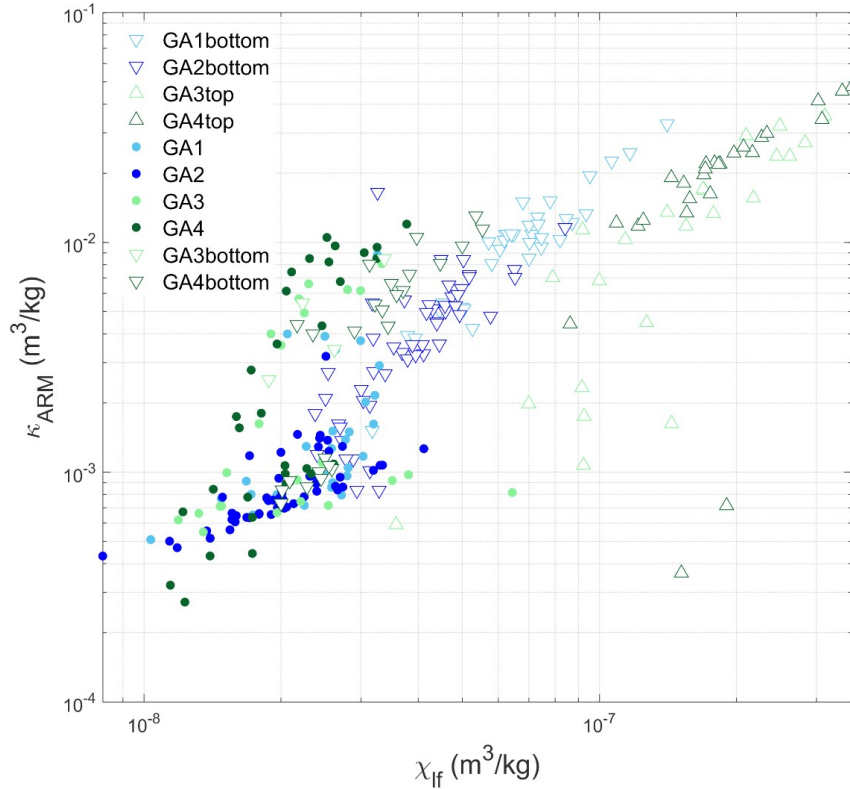
Figure 12. King plot of all the profiles considered in the study with a distinction of the top of GA3 and GA4 and bottom of GA1 and GA2. The bottom section of all four profiles shows a small grain size, the middle section larger particles and the top section a mid-size particles.
