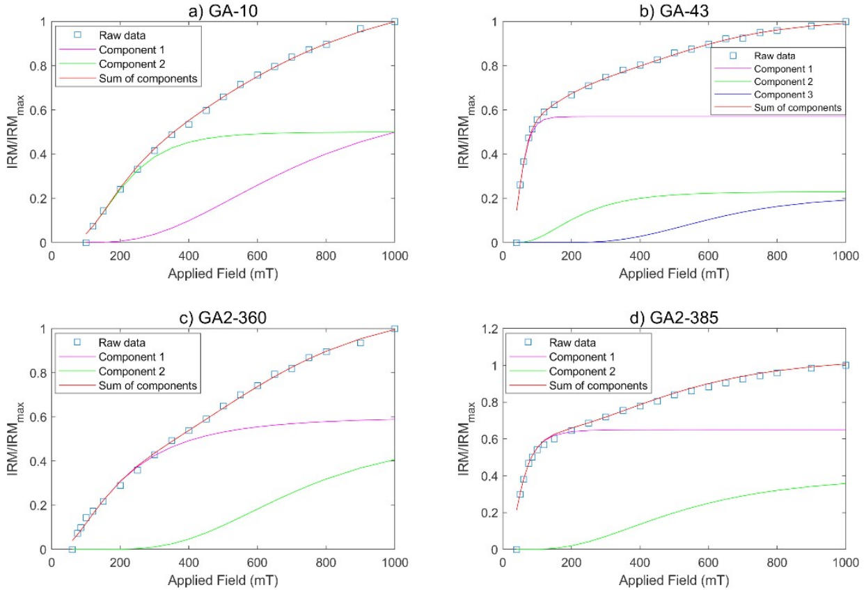
Figure 6. Analysis of the Linear Acquisition Plot (LAP) with the Kruiver approach of the samples illustrated in the IRM progressive acquisition. The squares represent the measured data of the IRM acquisition curve on a linear scale and the solid line is the modelled one (thin lines indicate the components derived from the model). The non-saturated samples of GA1 and GA2 are illustrated in (a) and (c). The saturated ones of the respective profiles are illustrated in (b) and (d).
