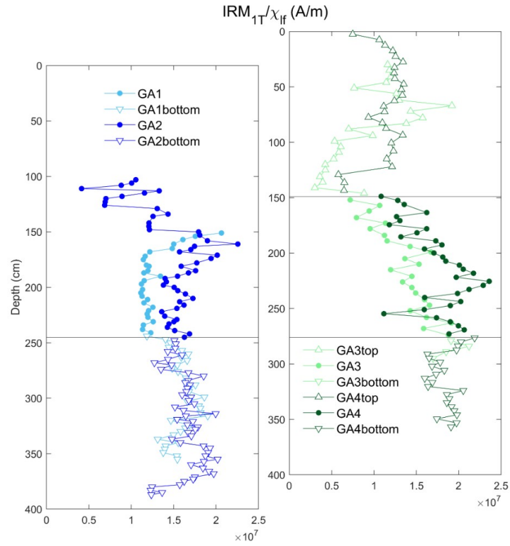
Figure 13. Magnetic grain size analysis with ratio IRM_{1T}/\chi_{lf} with respect to the depth: (a) GA1 and GA2; (b) GA3 and GA4.
