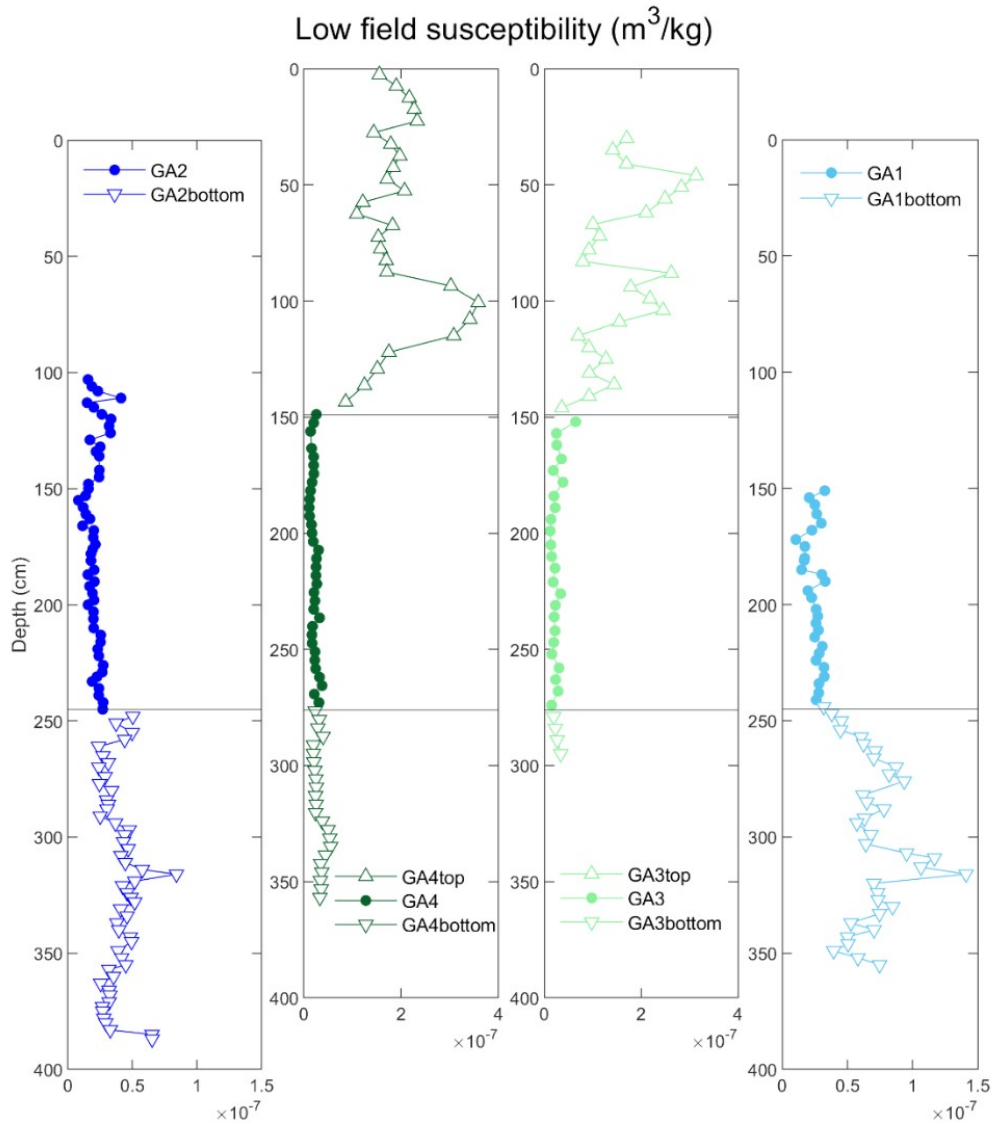
Figure 7. Low field susceptibility of all profiles analysed in the spatial correlation. Note the distinction of two intervals with higher values of susceptibility: the top of GA3 and GA4 profiles and the bottom of GA1 and GA2 profiles.
