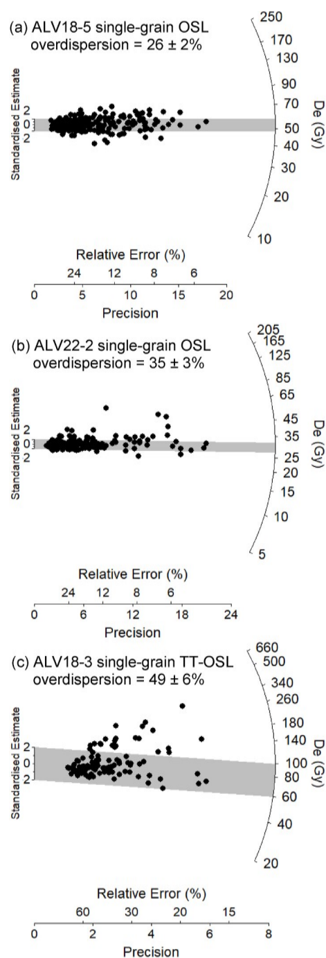
Fig. 2. Representative single-grain OSL and TT-OSL D_e distributions for the Lagar Velho dating samples, shown as radial plots. The grey bands on the radial plots are centred on the D_e values used for the age calculations, which were derived using either the central age model (CAM) for the single-grain OSL dataset of ALV18-5 or the 3-parameter minimum age model (MAM-3) for the single-grain OSL and TT-OSL datasets of ALV22-2 and ALV18-3. Individual D_e values that fall within the shaded region are consistent with the MAM-3 or CAM burial doses used for age calculation.
