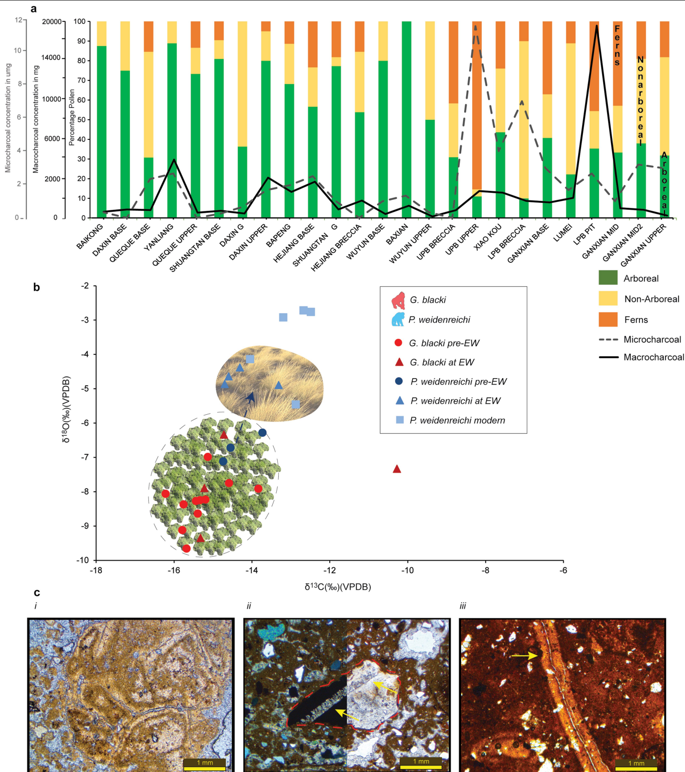
Extended Data Fig. 8 | Palaeoenvironmental proxies used in this study.
