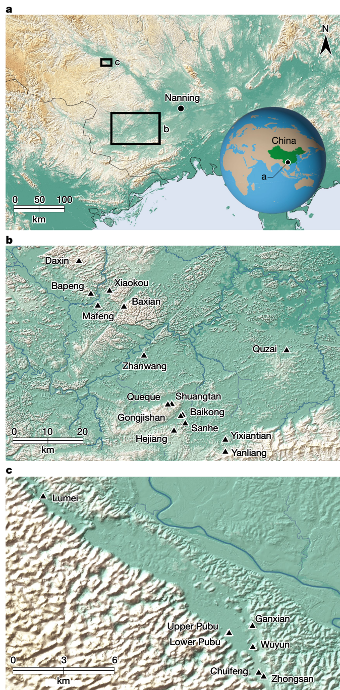
Fig. 1 | The location of the study sites in this research. a–c , The location of Southern China, Guangxi ZAR province and the city of Nanning ( a ), with the location of the Chongzuo study area marked by a large box ( b ) and the Bubing Basin study area marked by a smaller box ( c ). b , The location of the 16 cave sites analysed in the Chongzuo study area. c , The location of the six caves analysed in the Bubing Basin study area including both G. blacki -bearing and non- G. blacki -bearing caves from both regions.
