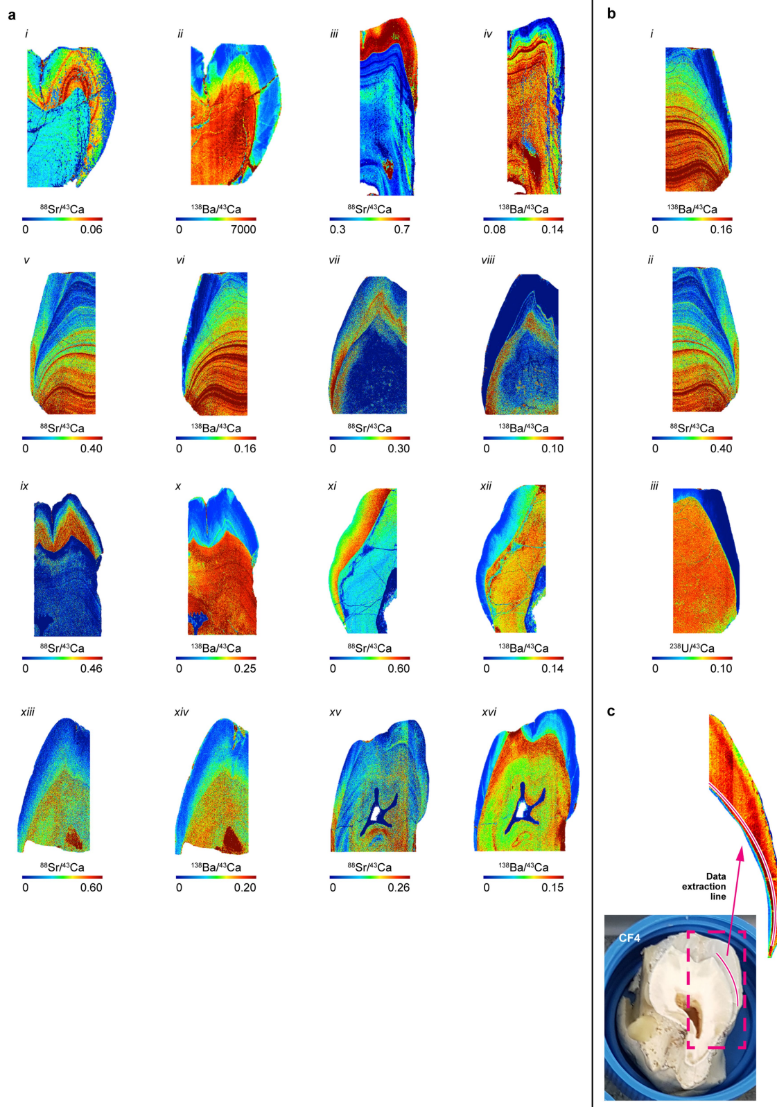
Extended Data Fig. 9 | A selection of strontium and barium elemental maps. Produced from Gigantopithecus blacki . Fossil teeth from various cave sites. a , i-ii : Chuifeng 1; iii-iv : Chuifeng 2; v-vi : Queque 44; vii-viii : Queque 5; xi-xii : Shuangtan 50; xiii-xiv : Shuangtan 109; xv-xvi : Hejiang 1573.8. b , Uranium as a
