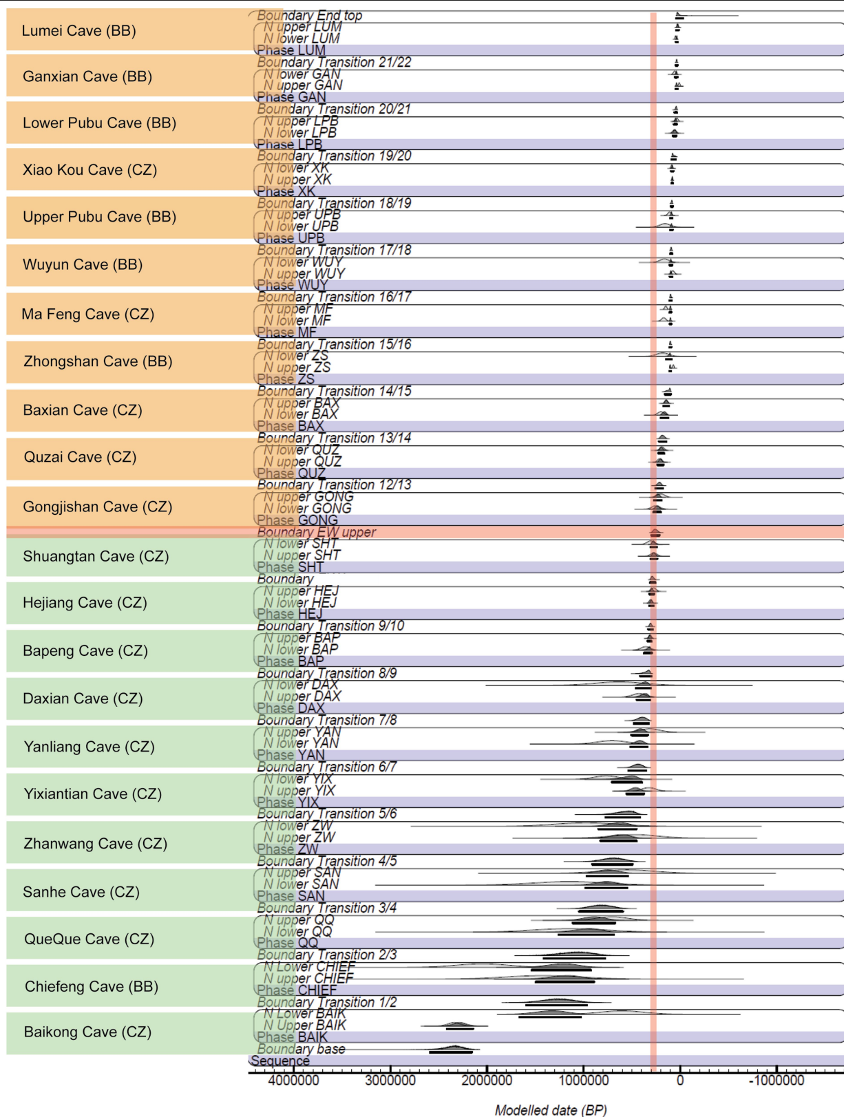
Extended Data Fig. 6 | Modelling of all 22 sites to establish the timing of the Extinction Window. The master Bayesian plot composed of the modelled age ranges for all 22 caves. The names of the caves have been included on the left – colour coded to signify the G. blacki -bearing caves (green) and the non- G. blacki -bearing caves (brown). Following each cave name its location is signified in brackets with either CZ – Chongzuo area or BB – Bubing Basin. See Fig. 1 for the
