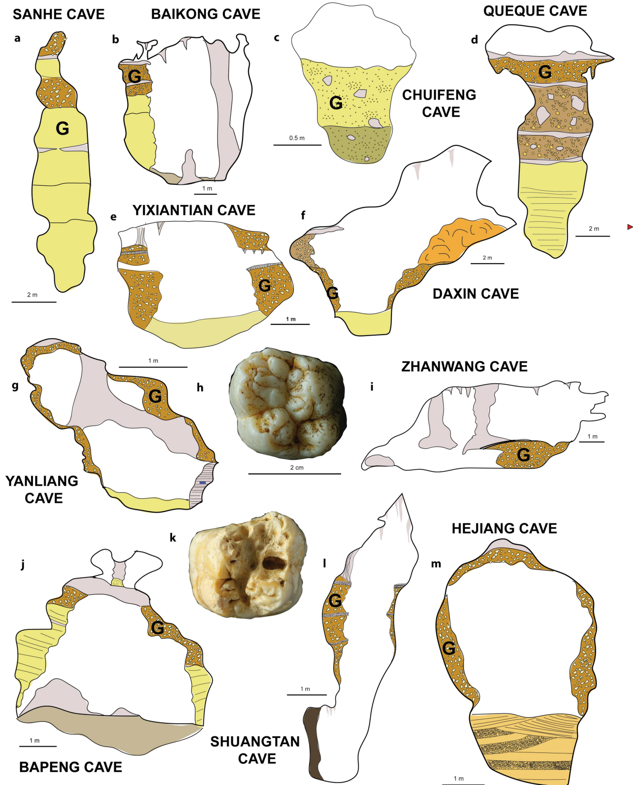
Extended Data Fig. 1 | The G. blacki caves in Chongzuo and Bubing Basin. a , Sanhe; b , Baikong; c , Chuifeng; d , Queque; e , Yixiantian; f , Daxin; g , Yanliang; h , a typical G. blacki teeth from older evidence from Sanhe cave; i , Zhanwang; j , Bapeng; k , a typical G. blacki teeth from younger evidence from Hejiang cave;
