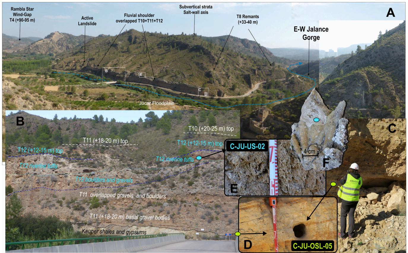
Fig. 13. Outcrops of the terraces T10, T11 and T12 on the left margin of the Júcar Valley between Rambla Star (North) and the Jalance Gorge (South). A) Panoramic view of the Júcar Valley showing the main geomorphological elements. B) View of the three terrace levels at the Júcar bridge site (El Puntal) with stacked deposits, showing the high-energy boulder gravel overlying unconformably the subvertical Triassic strata as well as the upper tufa deposits sampled for Th/U geochronological analysis. C) View of the sandy beds in the basal part of T11 sampled for OSL analysis (C-JU-OSL-05). D) Detailed view of the sediments sampled for OSL dating in T11. E) Detailed view of the tufa facies sampled for Th/U dating in T12. F) Dated tufa sample (C-JU-US-02) in phytoclast facies.
