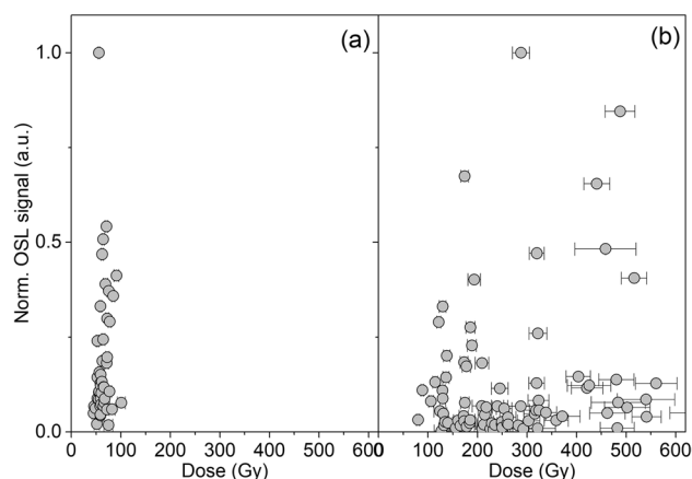
Fig. 4 Dose distributions of samples LM21140-1 (a) and LM21140-2 (b). The plots show the big differences between them. The large scatter observed on (b) is typical of a sample affected by incomplete bleaching
