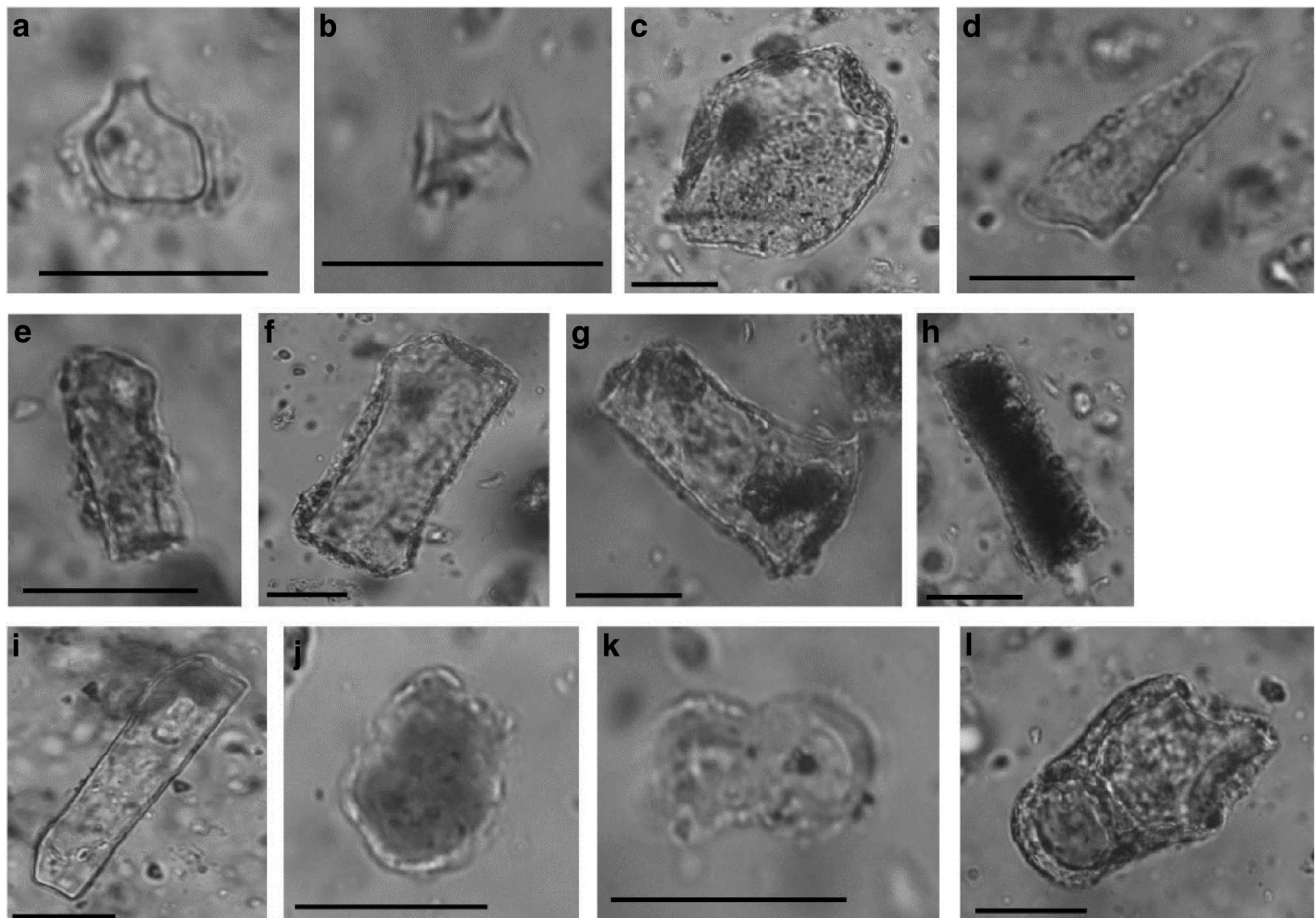
Fig. 17 Grass short cells: broken bilobate (a) and rondel (b). Grass bulliform type (c). Grass acicular hair cell (d). Blocky phytoliths (e, (f and g). Elongate: h and i. Globular/conical (j). Undetermined types from
