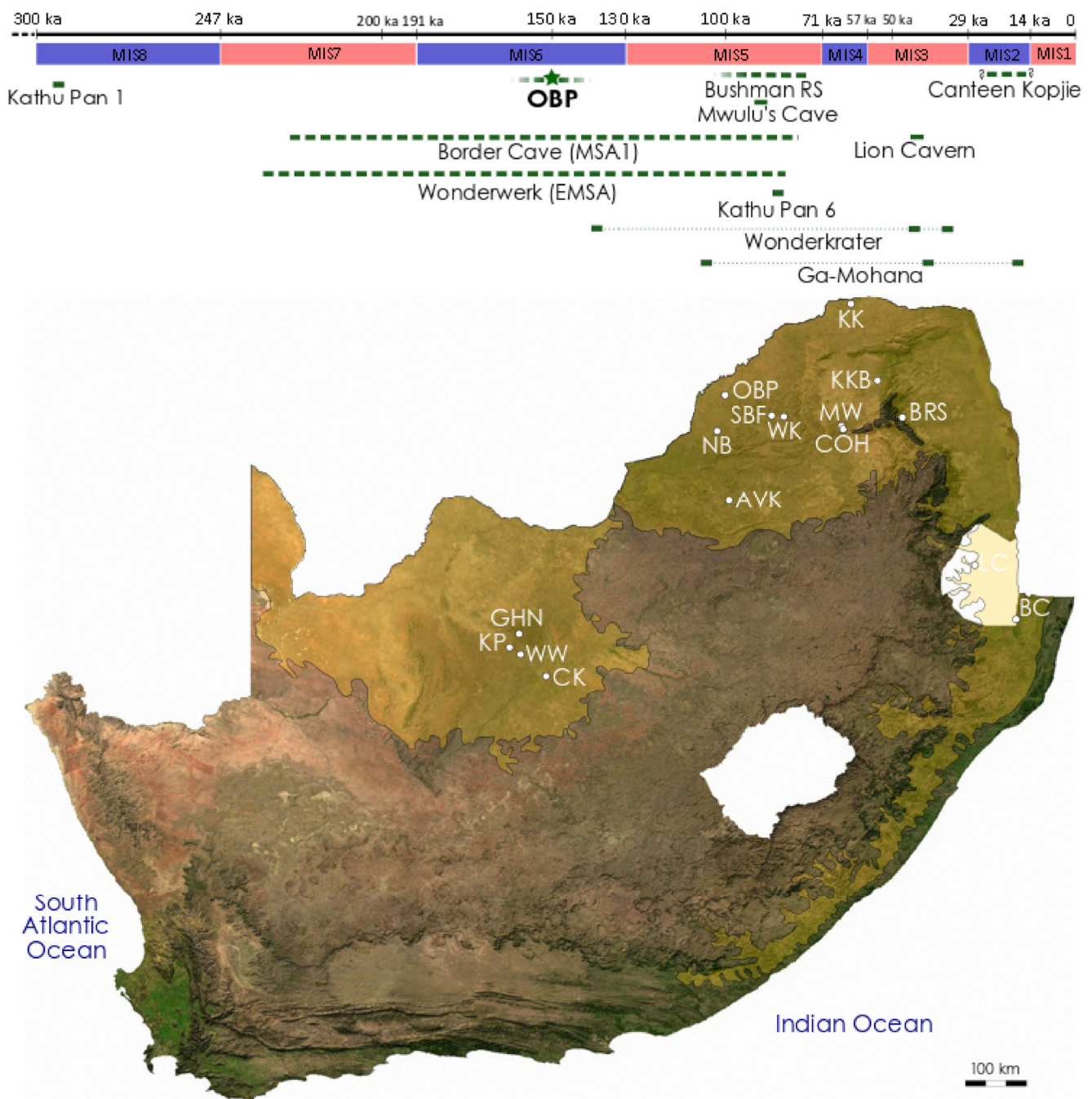
Fig. 18 Map of MSA sites located in the Savanna Biome (in light yellow) of South Africa, with existing dates for site occupation phases in this biome and the new dates for OBP. Abbreviations for site names are the following: AVK for Aasvoëlkop; BRS for Bushman Rock Shelter; CK for Canteen Kopje; COH for Cave of Hearths; GHN for Ga-Mohana Hill
