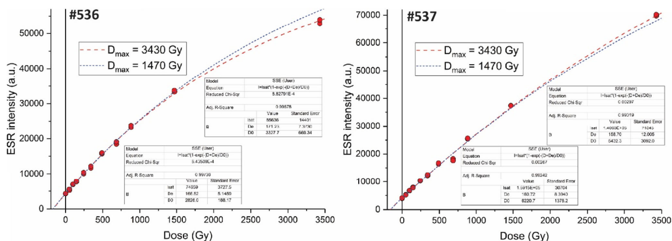
Fig. 15 ESR dose response curves obtained for the two samples. Fittings were performed over the full dose range ( D_{max} = 3430 Gy) and for a selected D_{max} of 1470 Gy in order to meet the recommendations by Duval and Grün (2016)
