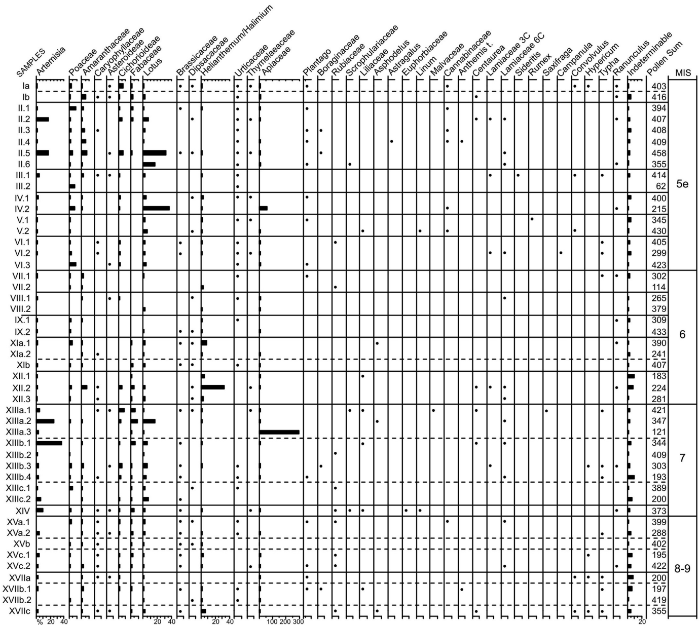
Fig. 7. Pollen diagram of Bolomor Cave including largely non arboreal elements Apiaceae , Ceratonia , Helianthemum / Halimium and Lotus out from the total pollen sum. Black dots for percentages below 3%. The dashed lines indicate subdivisions within a level.
